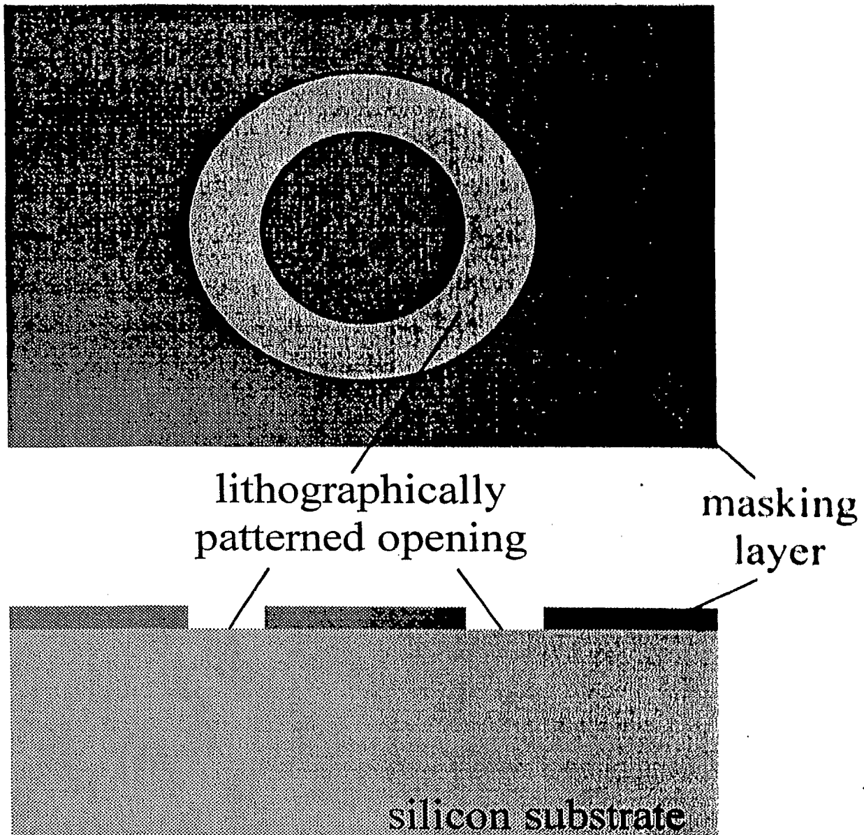
Fig. 4. Top and cross-sectional view of the annulus masking pattern.
